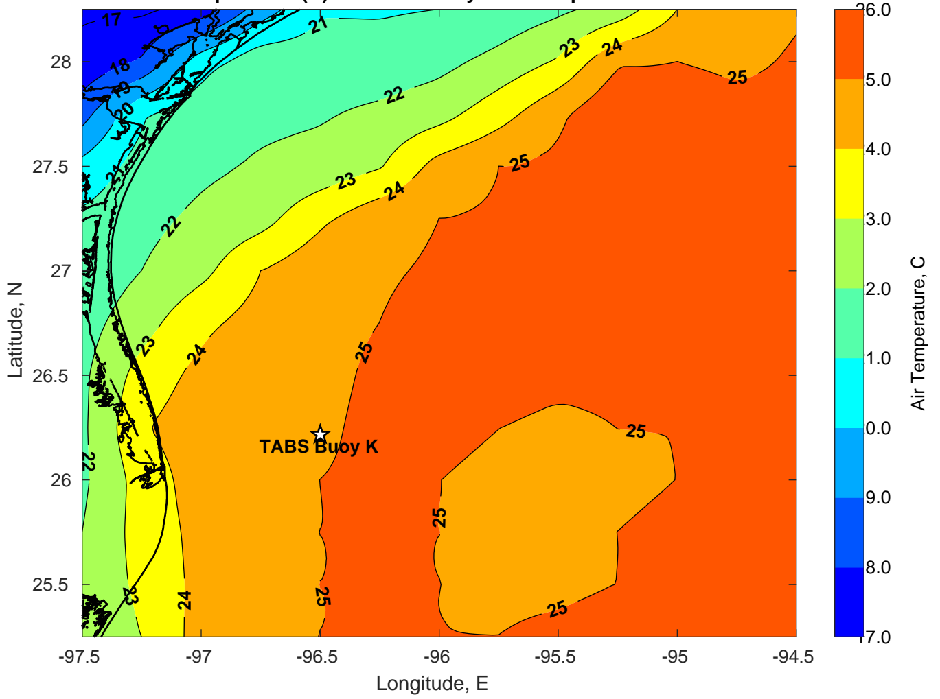
Air Temperature (C) for TABS Buoy K at 04-Apr-2023
